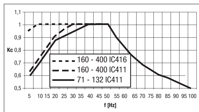
Curve 4: 4 poles - T4, T135°C
